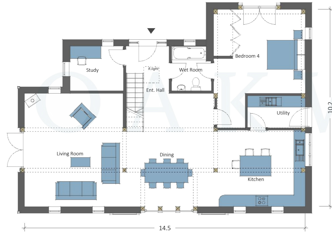
GROUND FLOOR GIA- 120 m 2
