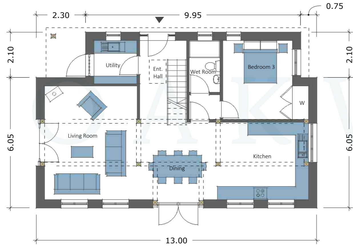
GROUND FLOOR GEA- 106.40m 2
