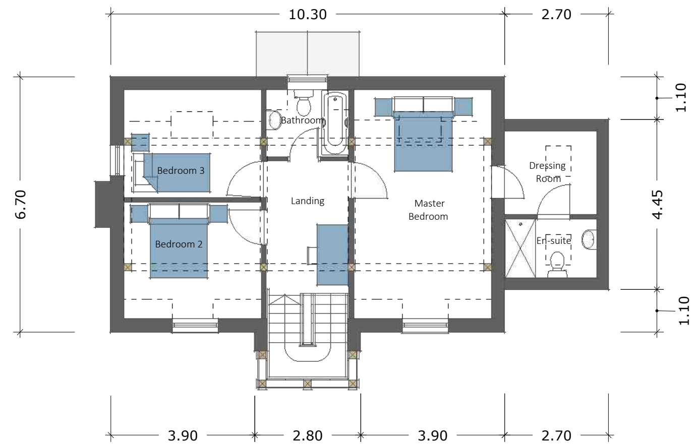
FIRST FLOOR GEA- 85.50 m 2
