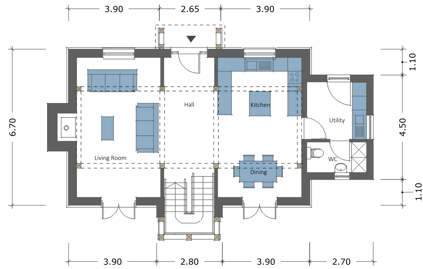
GROUND FLOOR GEA- 90.50 m 2
